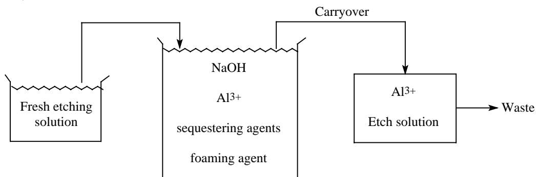
Figure 3 - The etching solution cycle
