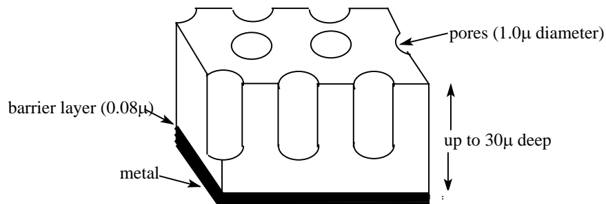
Figure 2 - Structure of anode layer
